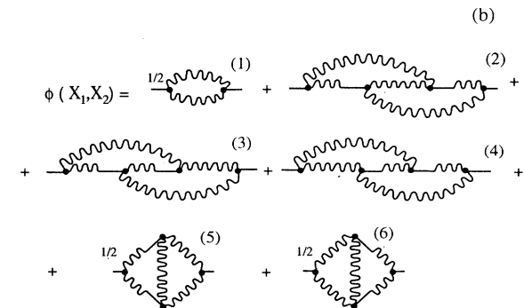
FIG. 2. Diagrammatic representation of the renormalized series expansion for the mass operators. (a) The mass operator \Sigma of the Dyson equation (2.8) and (b) the mass operator \Phi of the Wyld equation (2.9).
